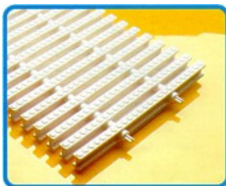
P1130/A Mod. GR/25 rigid grating; width mm. 250 x thickness mm. 25
