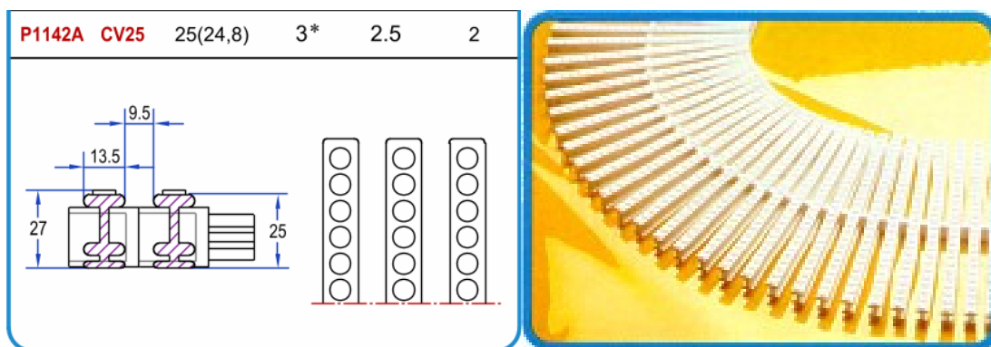
P1142/A Mod. CV/25 curvable grating; standard sizes: mm 250 x mm 25
